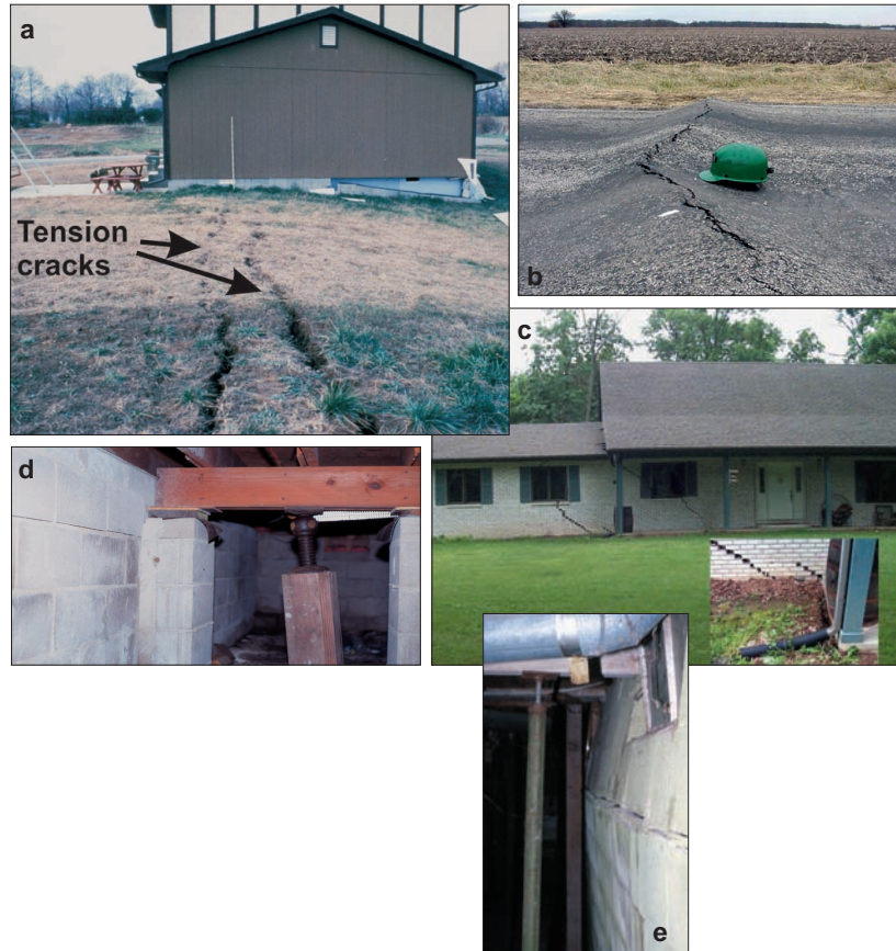
Front Cover: (a) Tension cracks formed in the ground surface extending through a home; the foundation has settled at the house corner closer to the center of sag. (b) Compression ridges formed in a road as the result of ground movement (compression) associated with coal mine subsidence. (c) The brick-sided house in the tension zone shows downward bending (compare roof lines). The left side of the home is closest to the sag center and has dropped down. Inset: ground has pulled away from the porch toward the sag center (left). (d) Settlement of the main beam caused by construction problems. (e) This basement damage was unrelated to mine subsidence. It was caused from decades of seasonal wetting and drying of soils, which built up pressure against the basement foundation walls. With each cycle, dryness allows fine grains of soil to fall into the gap between the soil and the foundation wall. When moisture returns, the soil expands, increasing pressure until the wall fails and is pushed inward.
