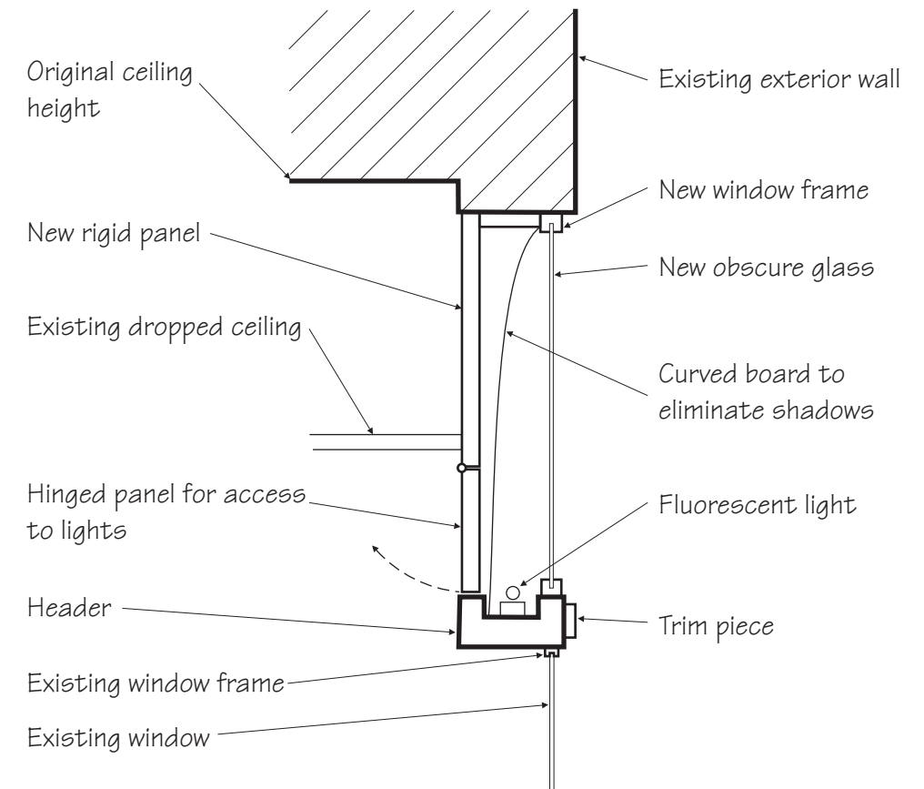
SCHEMATIC SECTION THROUGH TRANSOM
