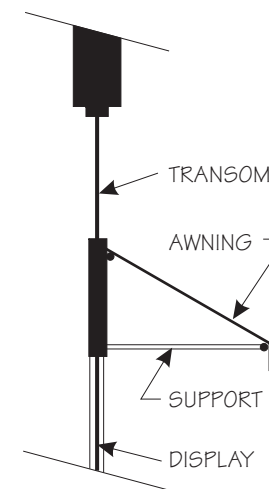
AWNING SECTION:
