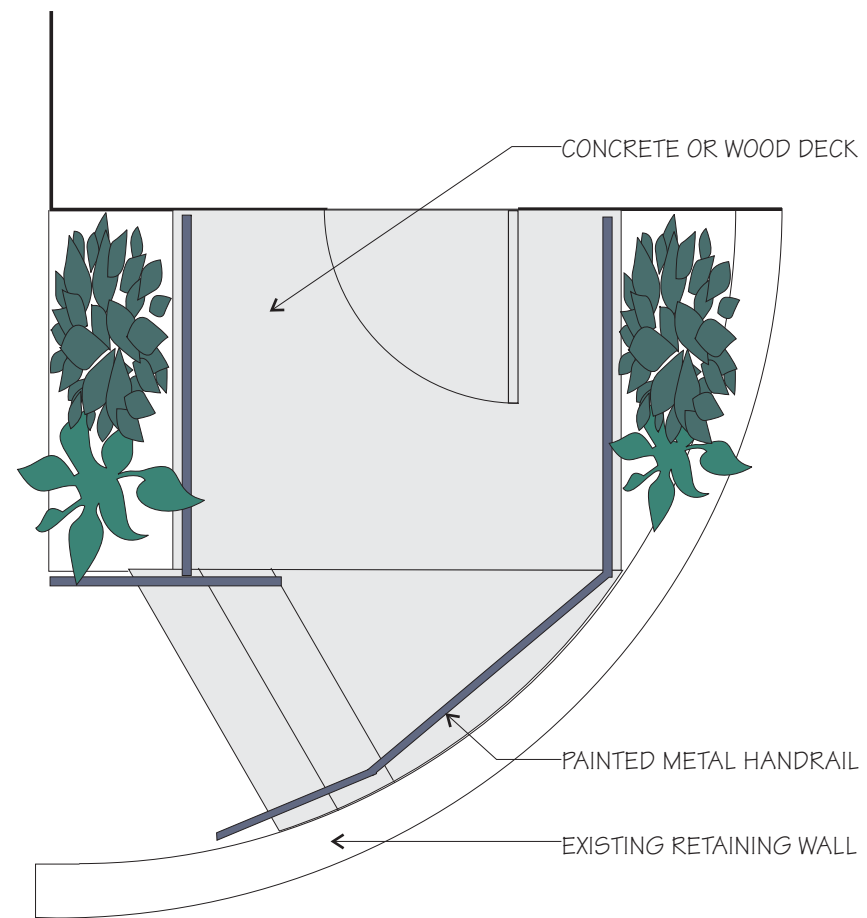
SCHEMATIC PLAN
