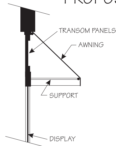
AWNING SECTION
