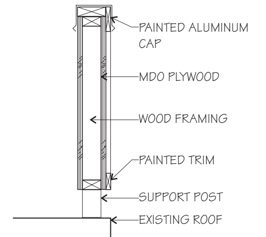
PARAPET SCREEN WALL
